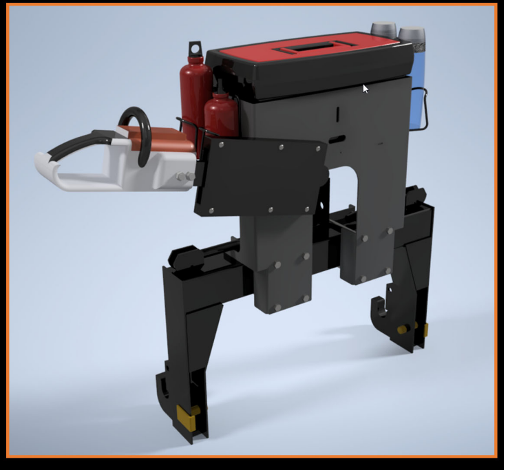
Tool Rack mounted on the Quick Hitch
